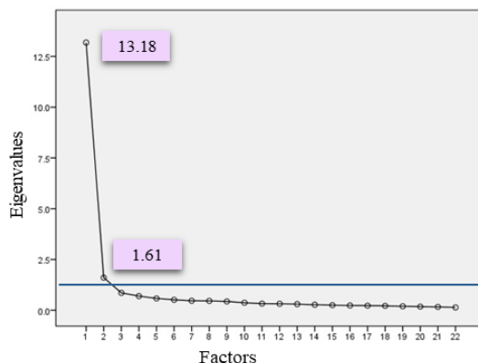
Figure 1. Scree plot of the factors of the Familiarity with the Qur'an Questionnaire in exploratory factor analysis
